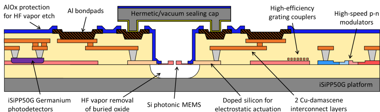
Figure 3. Cross section of photonic MEMS on the iSiPP50G foundry platform.
