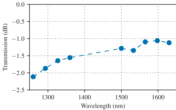
Fig. 7. Loss of a SiN fiber edge-coupler connected to an optical fiber Nufern UHNA4 fusion spliced to a G.652 fiber Corning SMF-28. The loss is determined by halving the measured fiber-to-fiber transmission of a waveguide integrated with 2 edge couplers and includes the 0.2 dB splicing loss.
