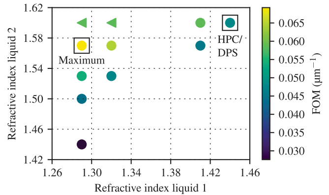
Fig. 2. FOM of SiN LCCs with liquid combinations of various refractive indices over the wavelength range 1260 nm to 1650 nm.
