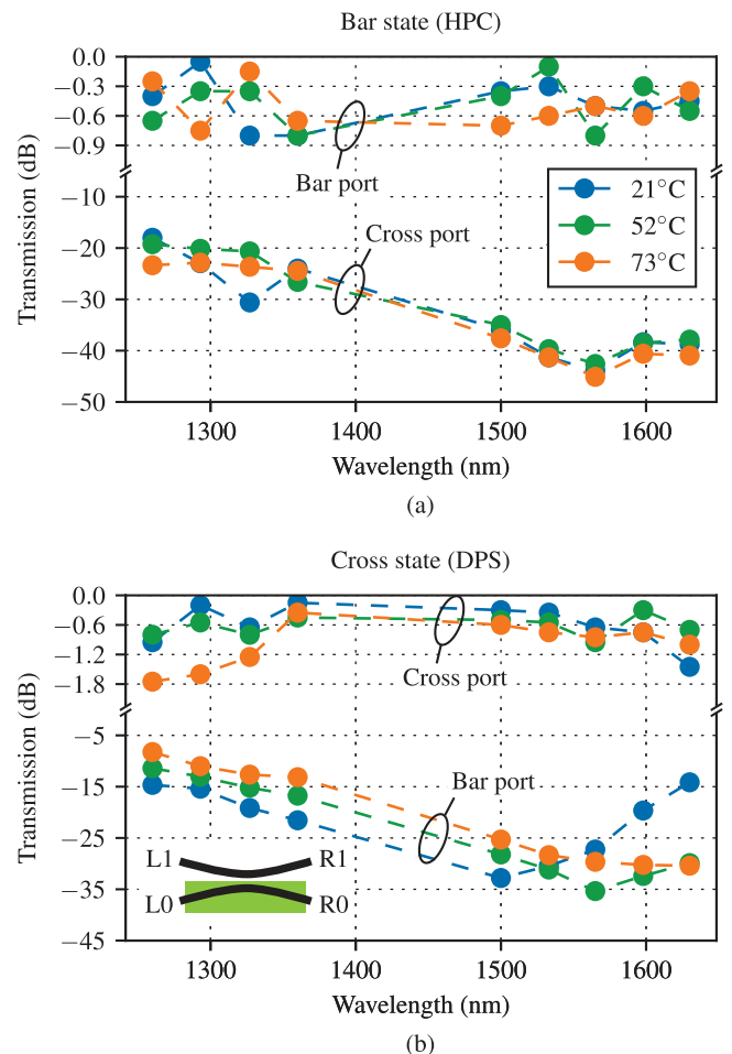
Fig. 6. Cross port and bar port transmission of a SiN LCC at different temperatures with input port L1; (a) bar state and (b) cross state.
