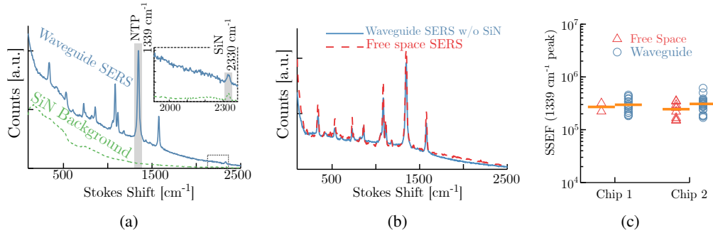
Fig. 5. (a) 4-NTP SERS signal acquired through the waveguide (solid blue) and the SiN background spectrum on a blank reference waveguide (dashed green). The 1339\text{ cm}^{-1} is used for quantifying the enhancement factor. The inset shows a characteristic peak for our SiN at 2330\text{ cm}^{-1} . (b) Waveguide collected SERS spectrum (solid blue) after subtracting the SiN background and scaling with the coupling losses, compared to a free-space collected SERS spectrum (dashed red) acquired on the same nanotriangle section. (c) SSEF for free-space excitation and collection compared to the signal strength using a waveguide-based measurement, acquired on multiple waveguides on two different chips.
