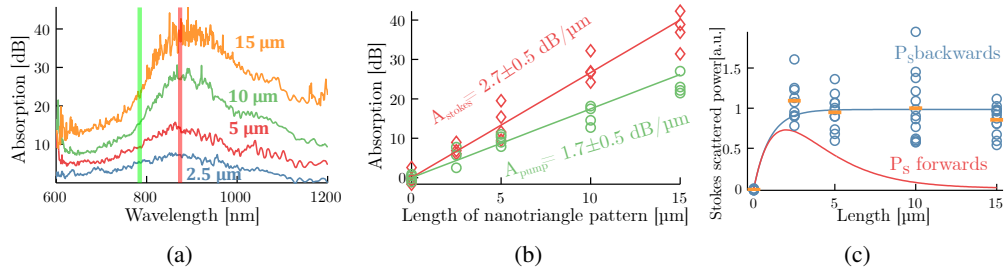
Fig. 3. (a) Absorption spectra of waveguides decorated with increasing lengths of nanotriangle patterns. The LSPR-absorption shows a good overlap with a 785 \text{ nm} pump laser and a 1139 \text{ cm}^{-1} Stokes shift, respectively green and red shaded. (b) Absorption versus nanotriangle length at pump and Stokes wavelength measured on four different waveguides for each length. A linear fit to the data gives an absorption of 2.7 \pm 0.5 \text{ dB}/\mu\text{m} at Stokes and 1.7 \pm 0.5 \text{ dB}/\mu\text{m} at the pump wavelength. (c) SERS signal strength in function of the length of the nanotriangle section, showing that the maximum signal is already reached for a 2.5 \mu\text{m} length. The orange bars give the average of at least 8 different measurements. The solid blue curve shows the calculated signal strength versus length when collecting the backwards Stokes scattered light in a reflection mode, as used in this work. The red curve shows the forward collected Stokes power in a transmission mode.
