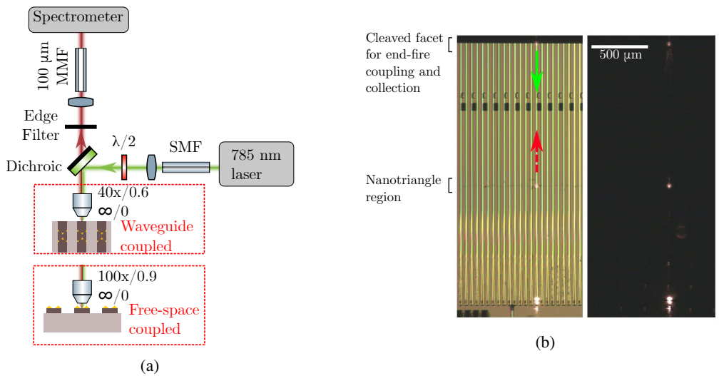
Fig. 4. (a) Schematic of the confocal microscope used for collecting Stokes scattered light from both waveguide- and free-space coupled nanotriangles. (b) Camera image of the chip in bright field (left) and dark field (right). Light is coupled from the top into the vertically oriented waveguides, and propagates along the waveguide (green arrow) until the nanotriangle section. Stokes scattered light is collected in reflection (red-dashed arrow). Scattering of the pump laser can be seen at the entrance facet and nanotriangle section.
