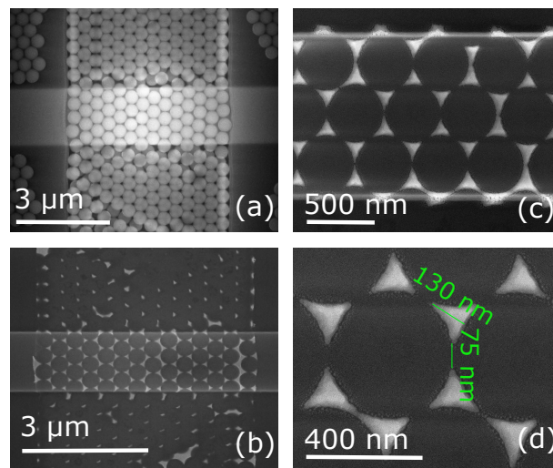
Fig. 2. SEM image of (a) a hexagonally close-packed monolayer of polystyrene beads in photoresist across the SiN waveguide and (b-d) a typical gold nanotriangle pattern on the waveguide.
