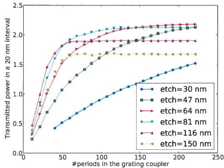
Figure 3: The total transmitted power in a 20 nm interval around the peak wavelength in function of the number of periods in the grating coupler for different etch depths. Normalized with respect to the grating coupler with an etch depth of 116 nm and 20 periods.
