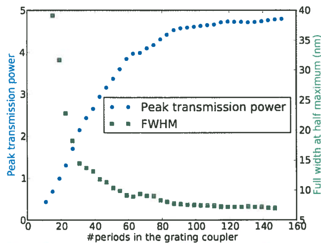
Figure 1: The peak transmission power and full width at half maximum of a grating coupler in function of number of periods. The former is normalized with respect to the grating coupler of 20 periods that is conventionally used for coupling light from optical fibers.
