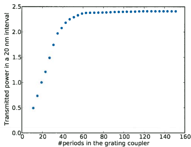
Figure 2: The total transmitted power in a 20 nm interval around the peak wavelength in function of the number of periods in the grating coupler, normalized with respect to the grating coupler of 20 periods.
