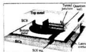
Figure 1. Schematic of microdisk resonator
