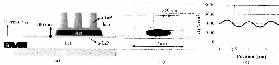
Figure 2: (a) The gallery waveguide structure of a bonded InP-based P-I-N laser. (b) The corresponding mode profile. (c) Current injection profile through the active layer.
