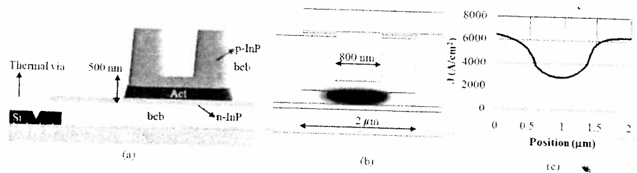
Figure 3: (a) The viking helmet waveguide structure of a bonded InP-based P-I-N laser. (b) The corresponding mode profile. (c) Current injection profile through the active layer.
