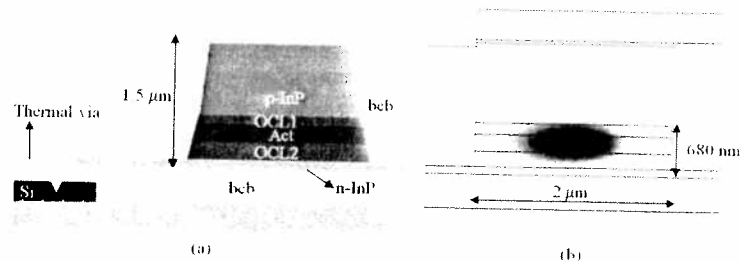
Figure 1: (a) The standard structure of a bonded InP-based P-I-N laser waveguide. (b) The corresponding mode profile.
