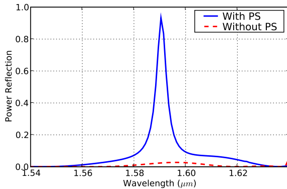
Fig. 2. Reflection spectra with and without a phase section (PS).
