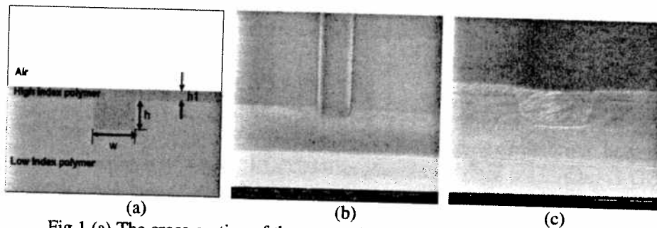
Fig.1 (a) The cross-section of the waveguide (b) SEM picture of the imprinted low index layer (c) SEM picture of waveguide cross-section (after spin-coating the high index layer)
