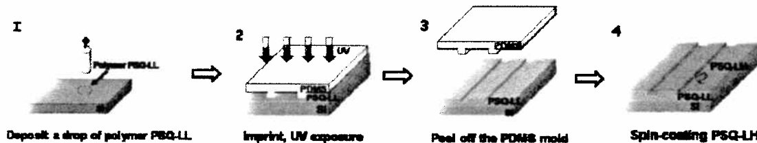
Fig.2 Fabrication process flow of the polymer waveguides
