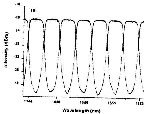
Fig.3 Measured transmission spectrum of microring resonator for TE polarized light
