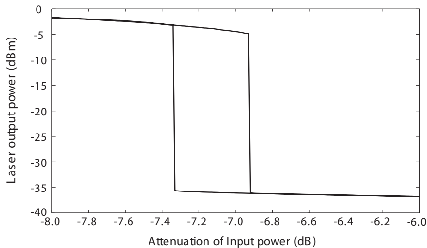
Figure 4: First experimental results on a \lambda/4 -shifted laser with length 510 \mu\text{m} and I_{\text{bias}} = 220\text{mA} .
