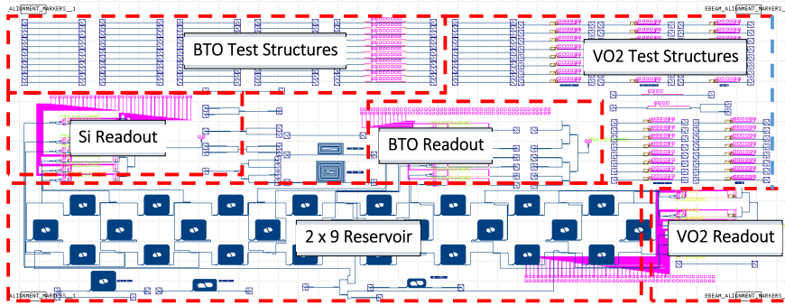
Figure 6.6: Mask plan for the silicon photonics chip consisting of a 2 \times 9 passive swirl photonic reservoir, and three readouts : a silicon readout, a VO_2 readout and a BTO readout as demarcated in the figure. The rest of the chip has different test structures to test passives components used in the reservoir and components to develop the BTO and VO_2 optical weighting elements.
