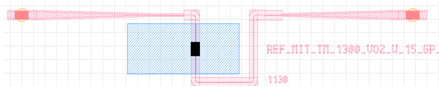
Figure 6.3: An example of a straight waveguide structure used to characterize the loss and characteristics of the metal-insulator transition. Red areas correspond to the silicon photonic structures while the blue ones correspond to the metallic contacts for the VO 2 stripes (marked in black).
